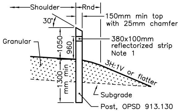
WOODEN DELINEATOR POST
